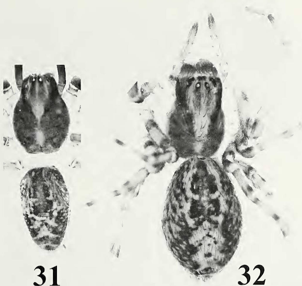
Figures 31, 32.— Taira sichuanensis new species, male holotype (31) and female paratype (32) from Changning, Sichuan, China, photos, habitus, dorsal view.
